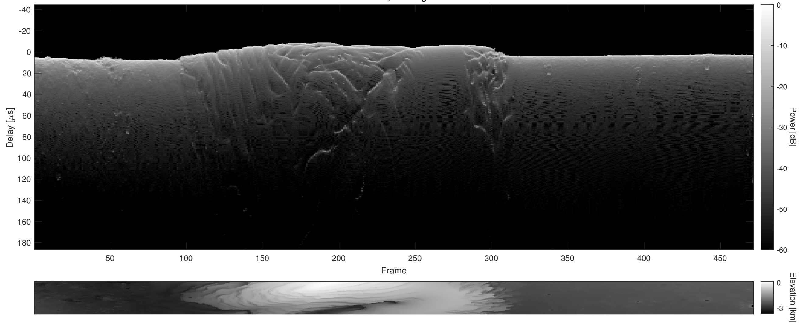
Orbit 5425, Cluttergram
