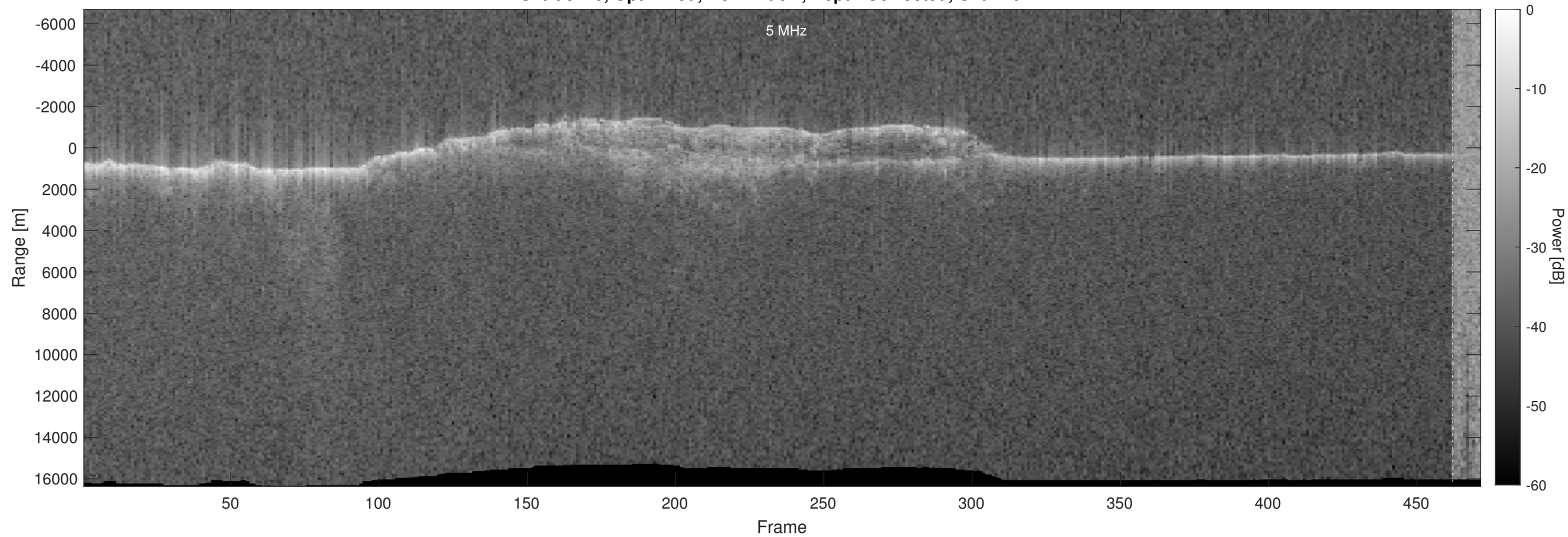
Orbit 5425, Optimized, No Window, Depth-Corrected, Channel 2
