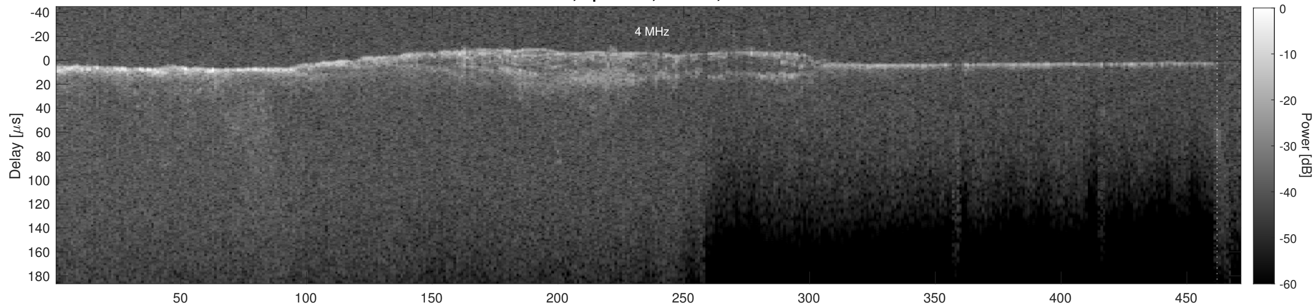
Orbit 5425, Cluttergram
