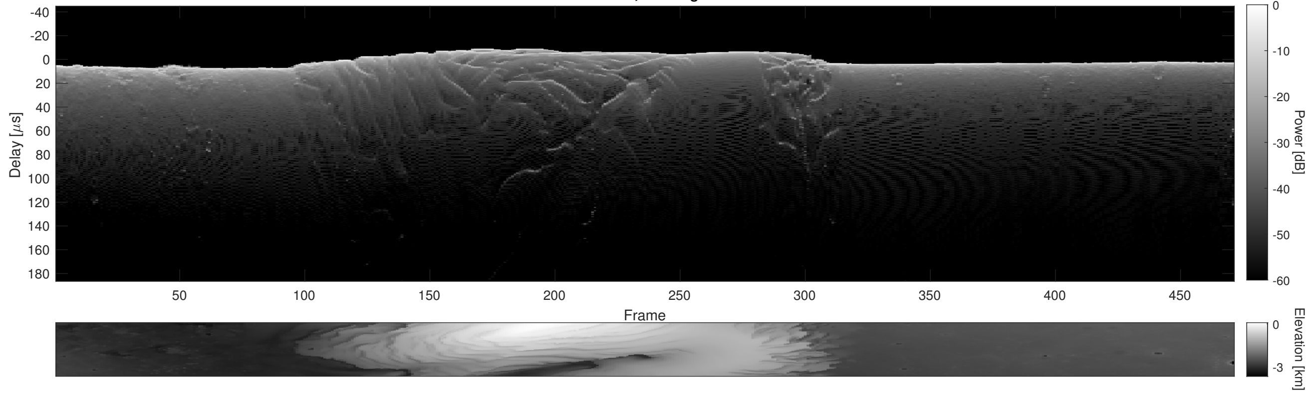
Orbit 5425, Cluttergram
