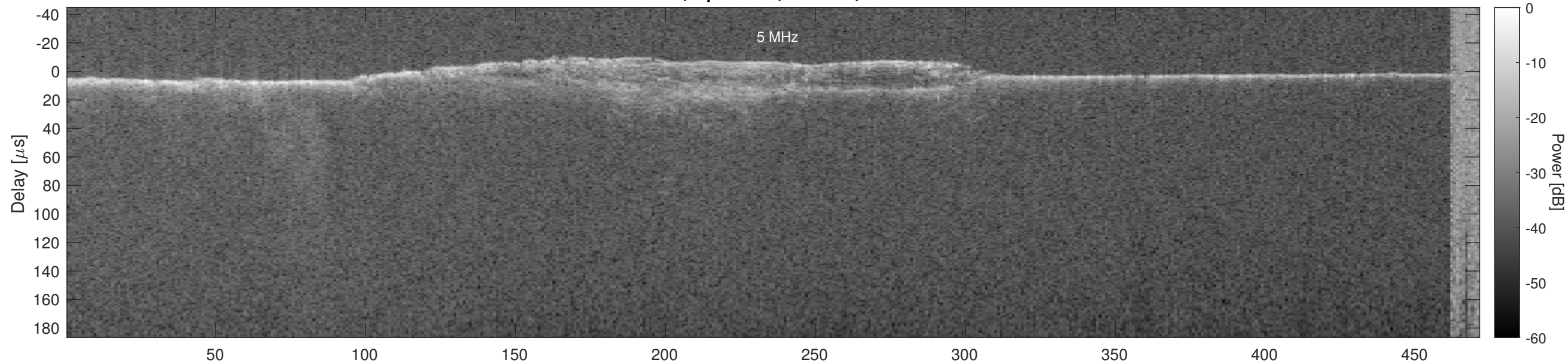
Orbit 5425, Optimized, Window, Channel 2
