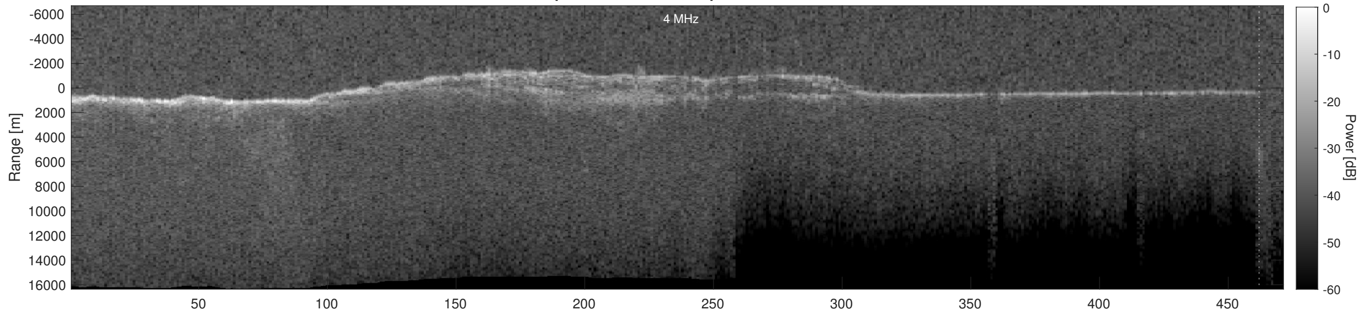
Orbit 5425, Depth-Corrected Cluttergram
