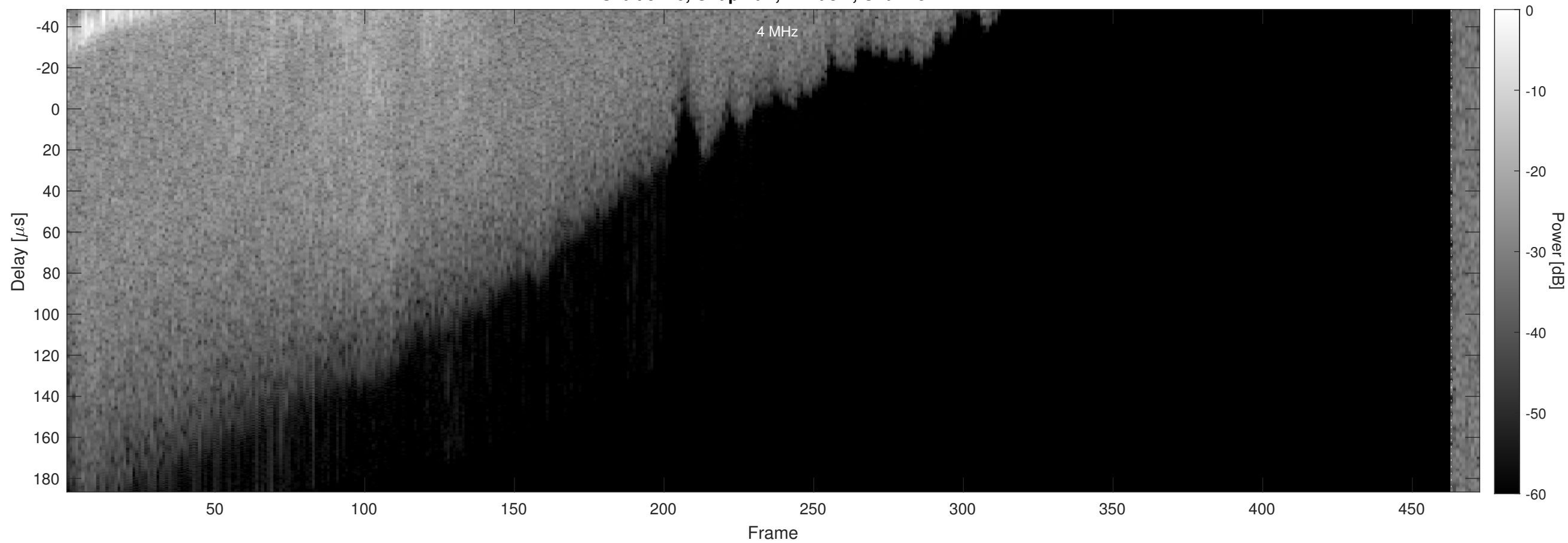
Orbit 5426, Chapman, Window, Channel 2
