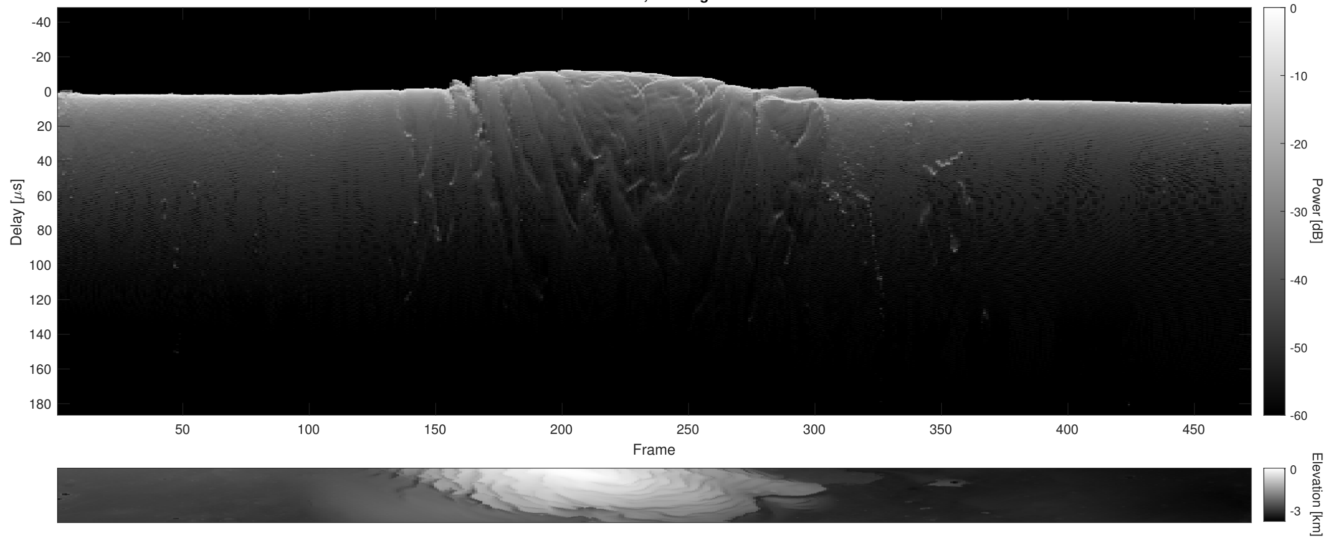
Orbit 5426, Cluttergram
