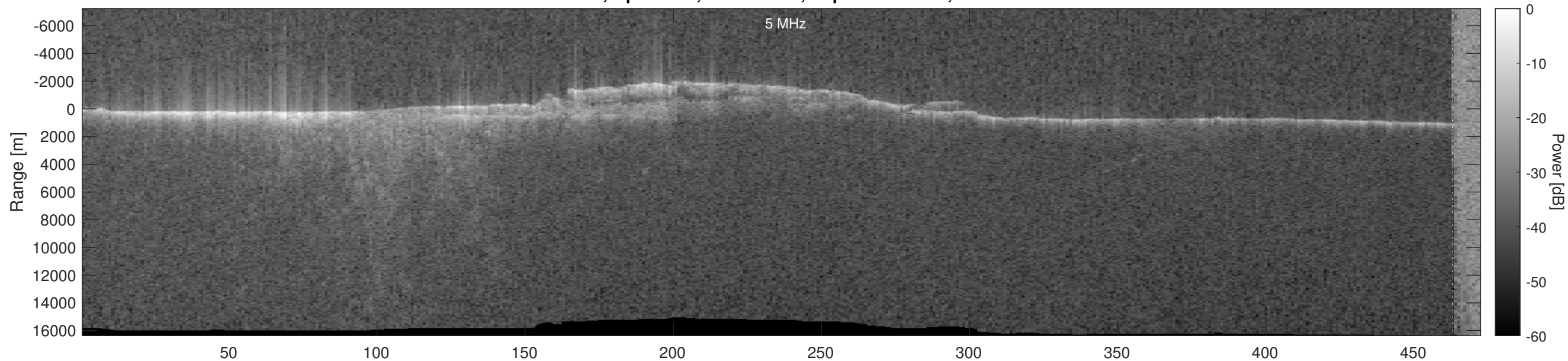
Orbit 5426, Optimized, No Window, Depth-Corrected, Channel 2
