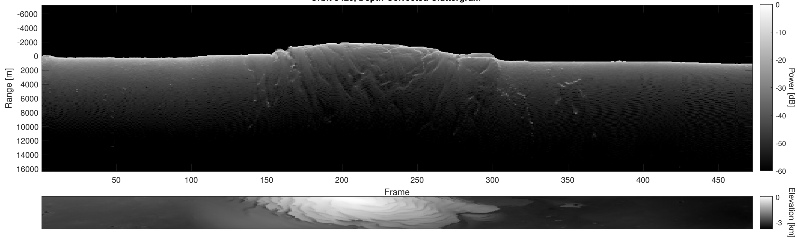
Orbit 5426, Depth-Corrected Cluttergram
