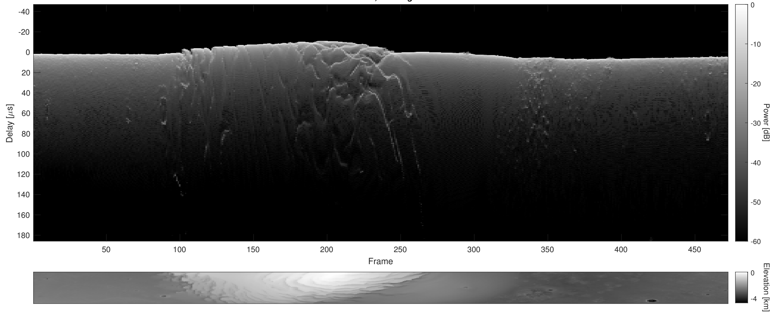
Orbit 5427, Cluttergram
