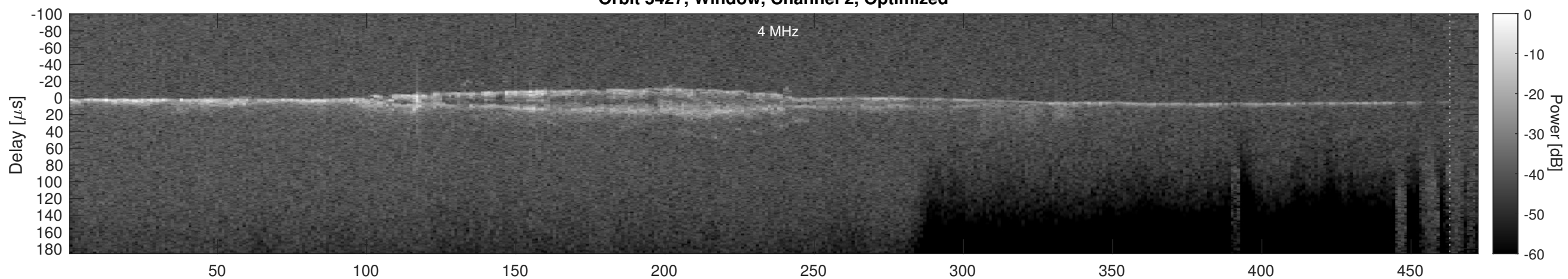
Orbit 5427, Cluttergram
