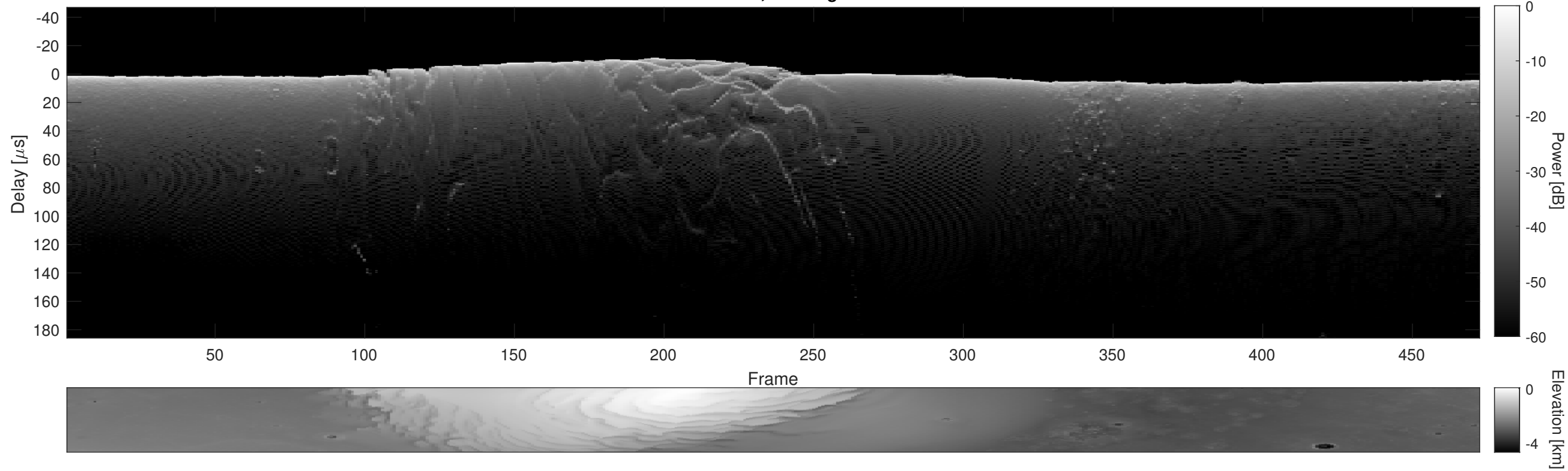
Orbit 5427, Cluttergram
