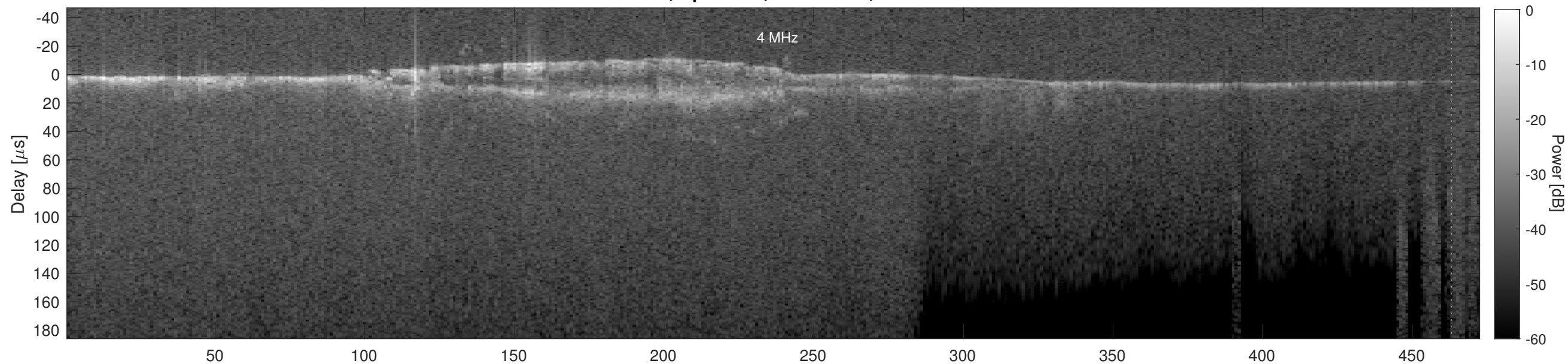
Orbit 5427, Cluttergram
