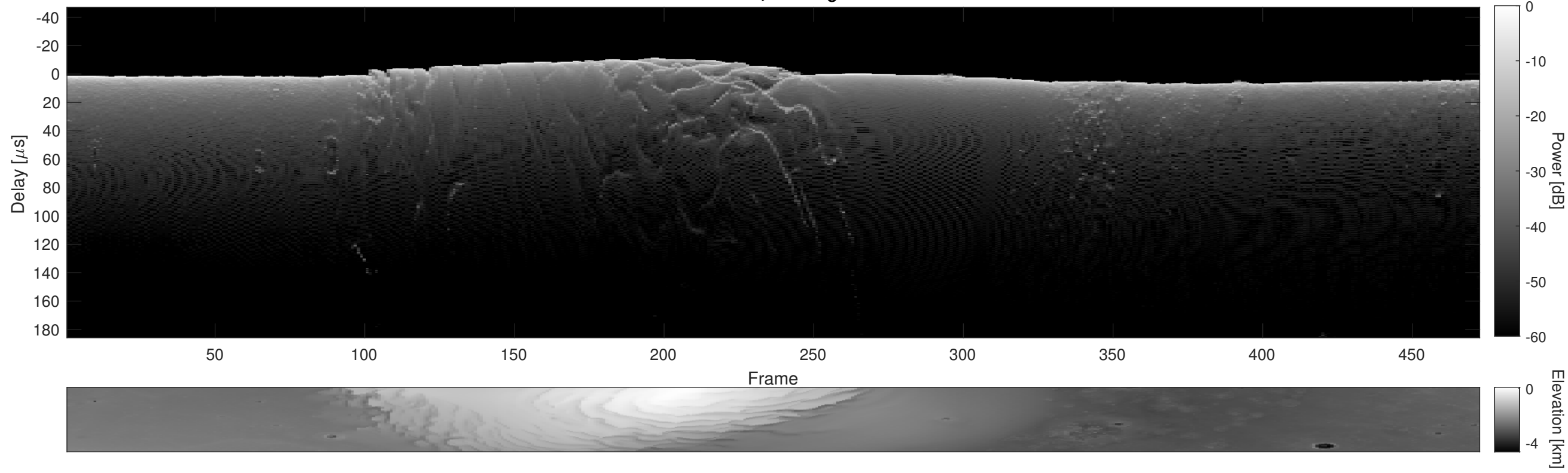
Orbit 5427, Cluttergram
