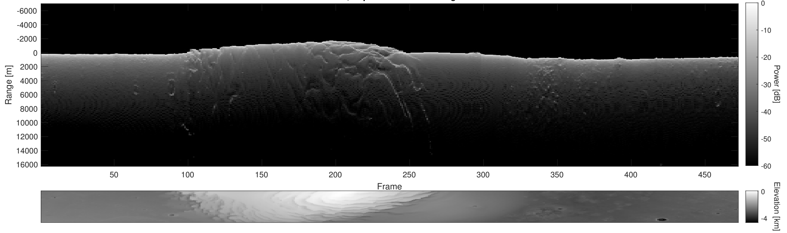
Orbit 5427, Depth-Corrected Cluttergram
