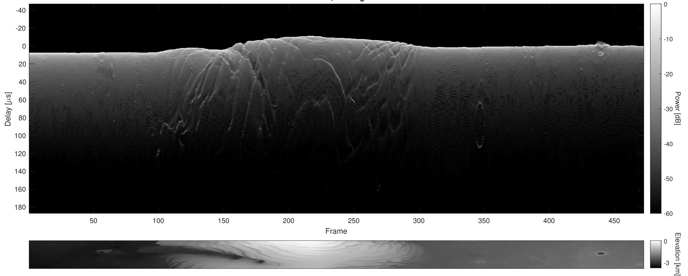
Orbit 5428, Cluttergram
