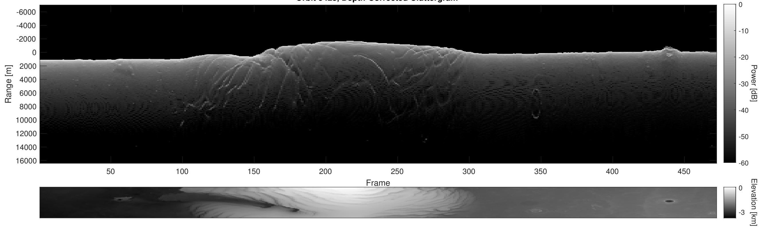
Orbit 5428, Depth-Corrected Cluttergram
