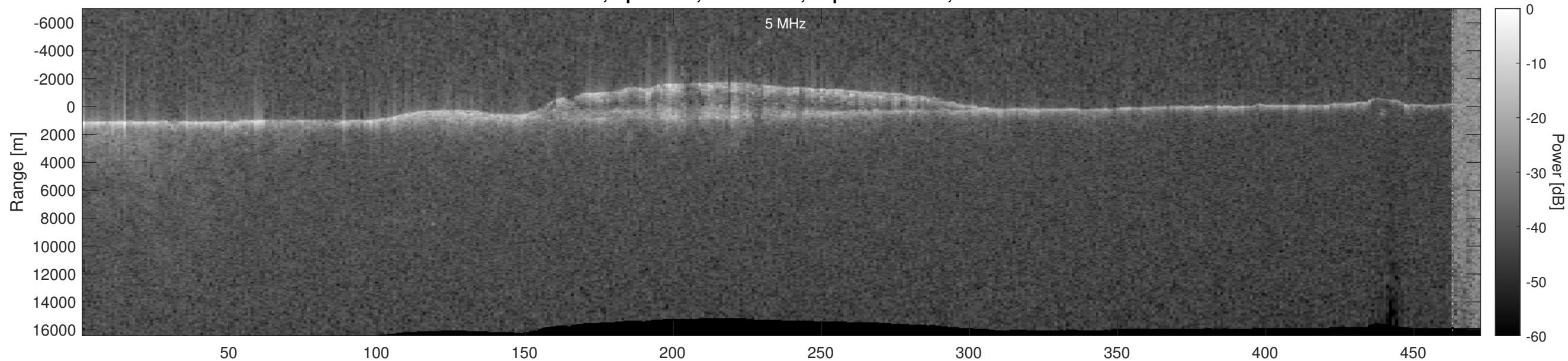
Orbit 5428, Optimized, No Window, Depth-Corrected, Channel 2
