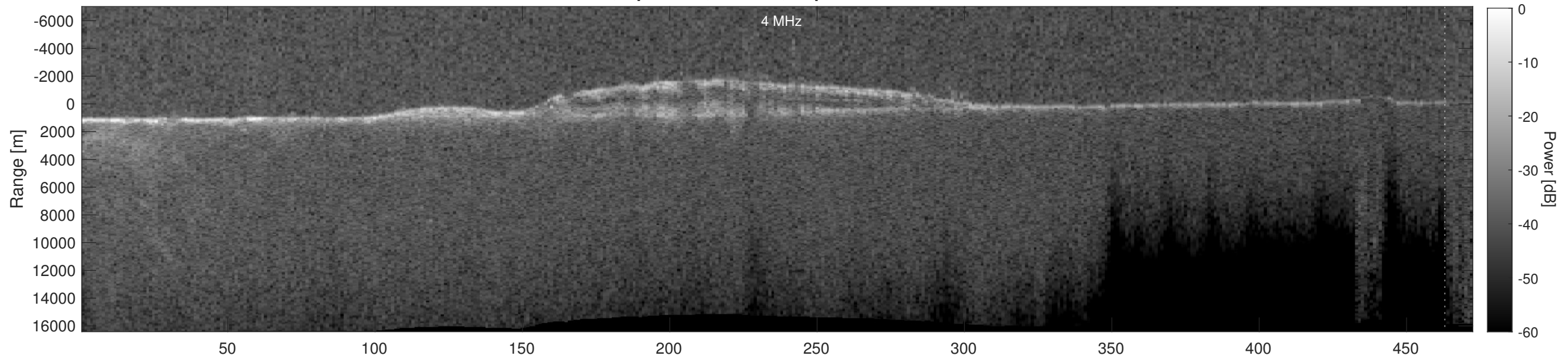
Orbit 5428, Depth-Corrected Cluttergram
