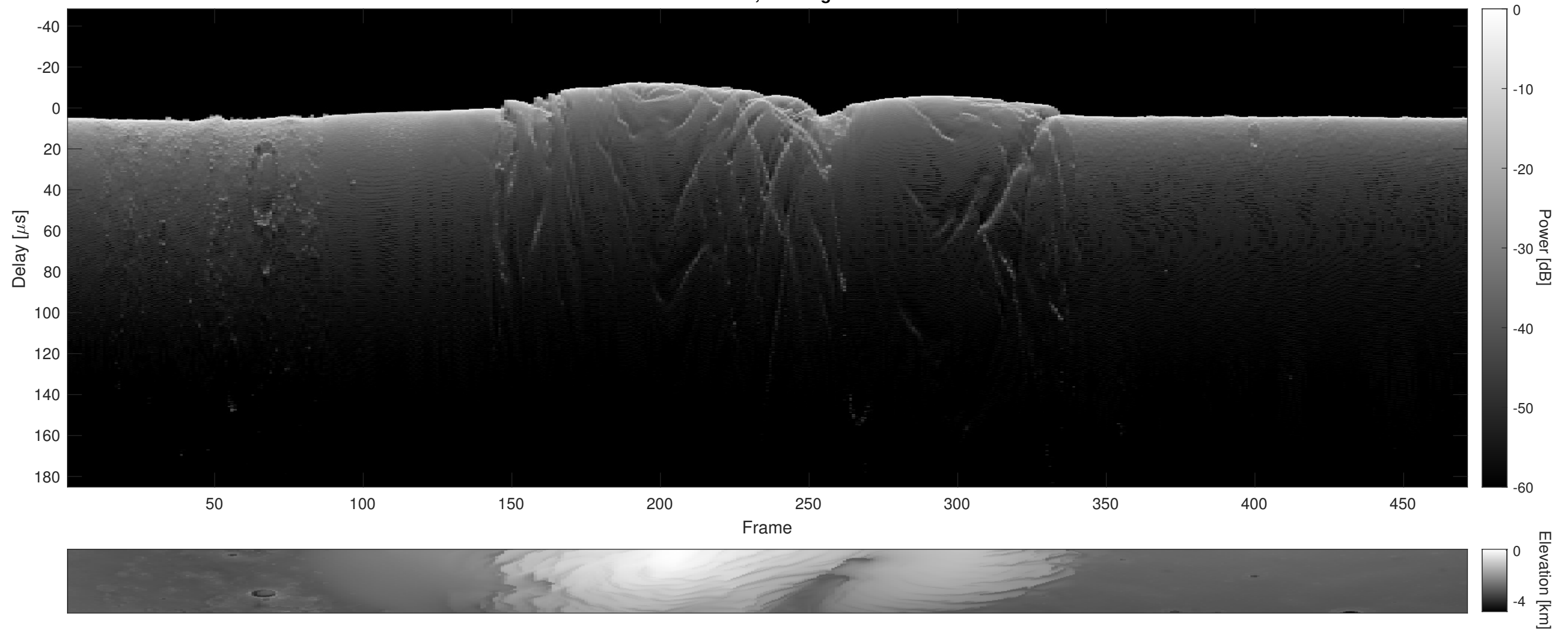
Orbit 5429, Cluttergram
