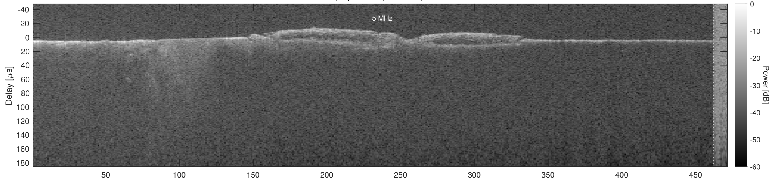
Orbit 5429, Optimized, Window, Channel 2
