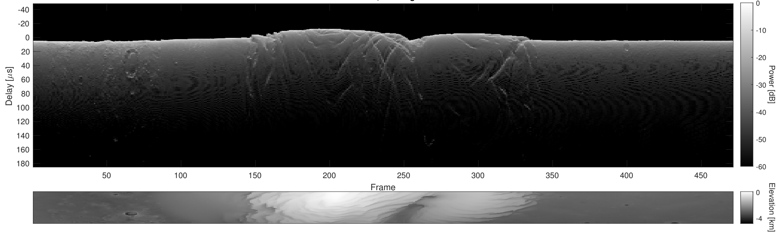
Orbit 5429, Cluttergram
