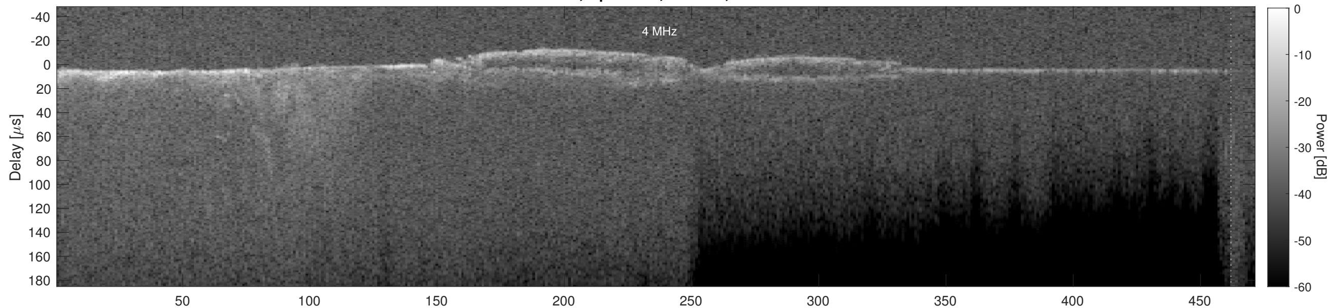
Orbit 5429, Cluttergram
