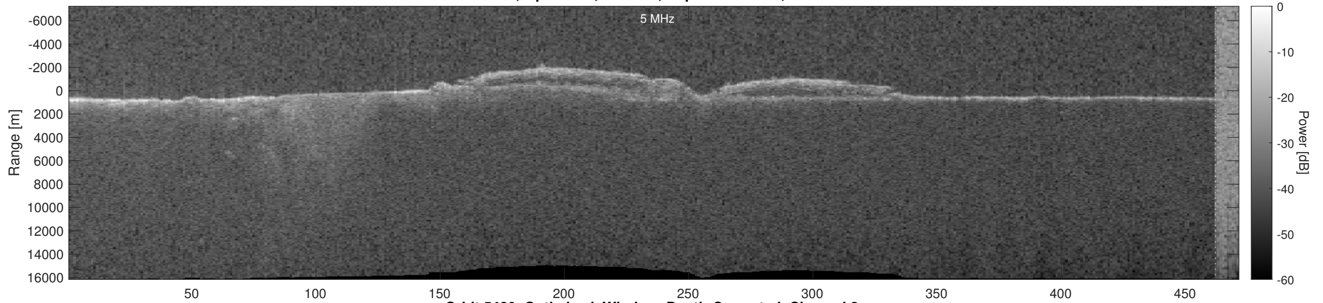
Orbit 5429, Optimized, Window, Depth-Corrected, Channel 2
