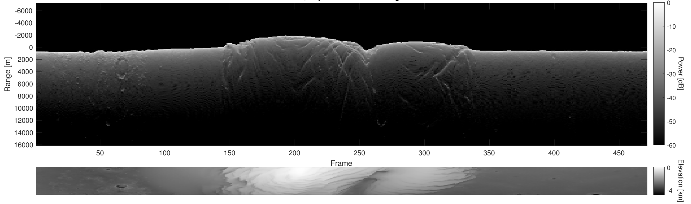
Orbit 5429, Depth-Corrected Cluttergram
