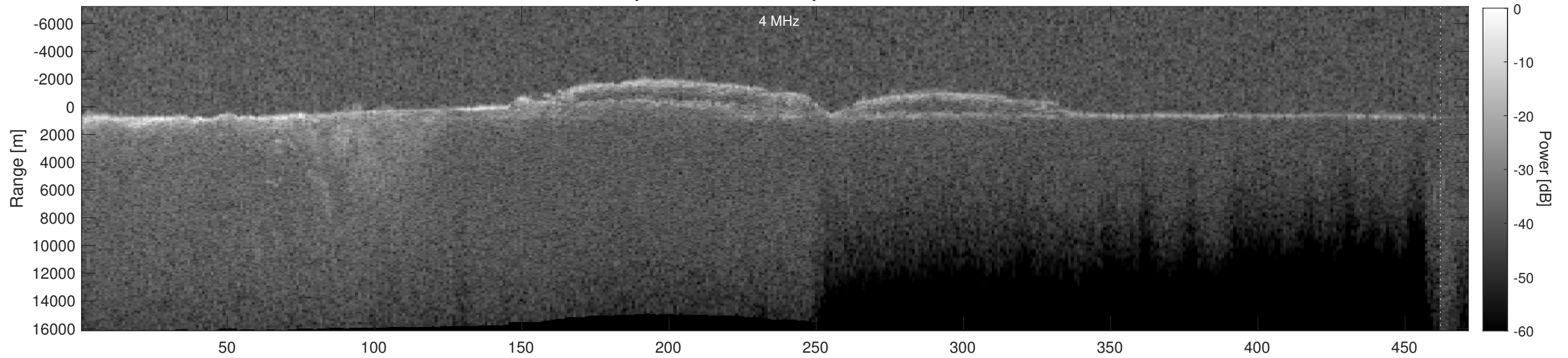
Orbit 5429, Depth-Corrected Cluttergram
