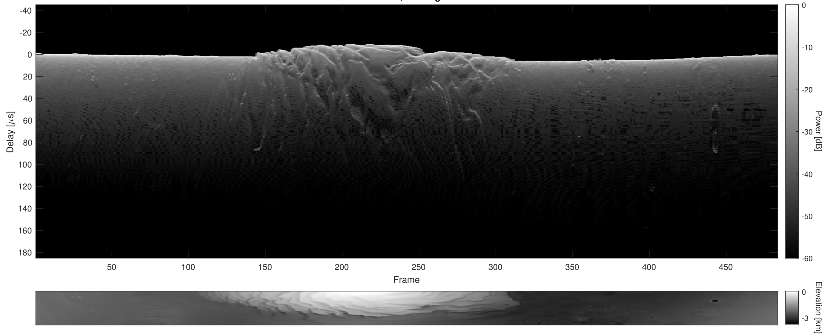
Orbit 5430, Cluttergram
