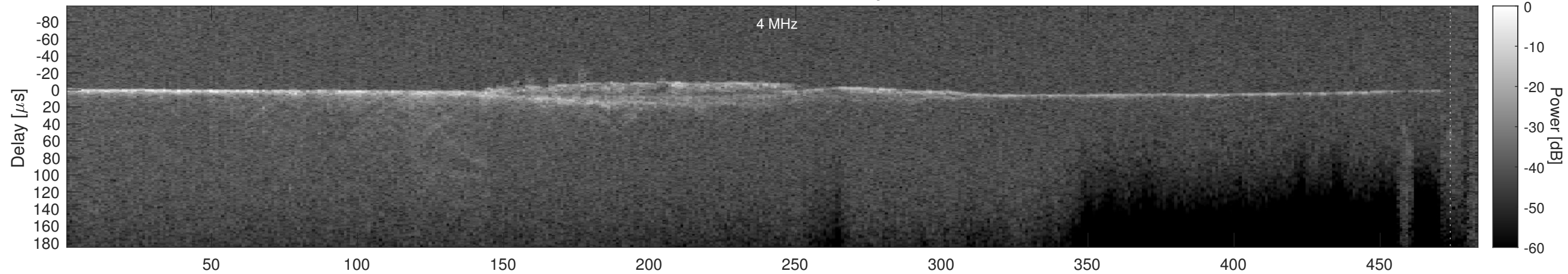
Orbit 5430, Cluttergram
