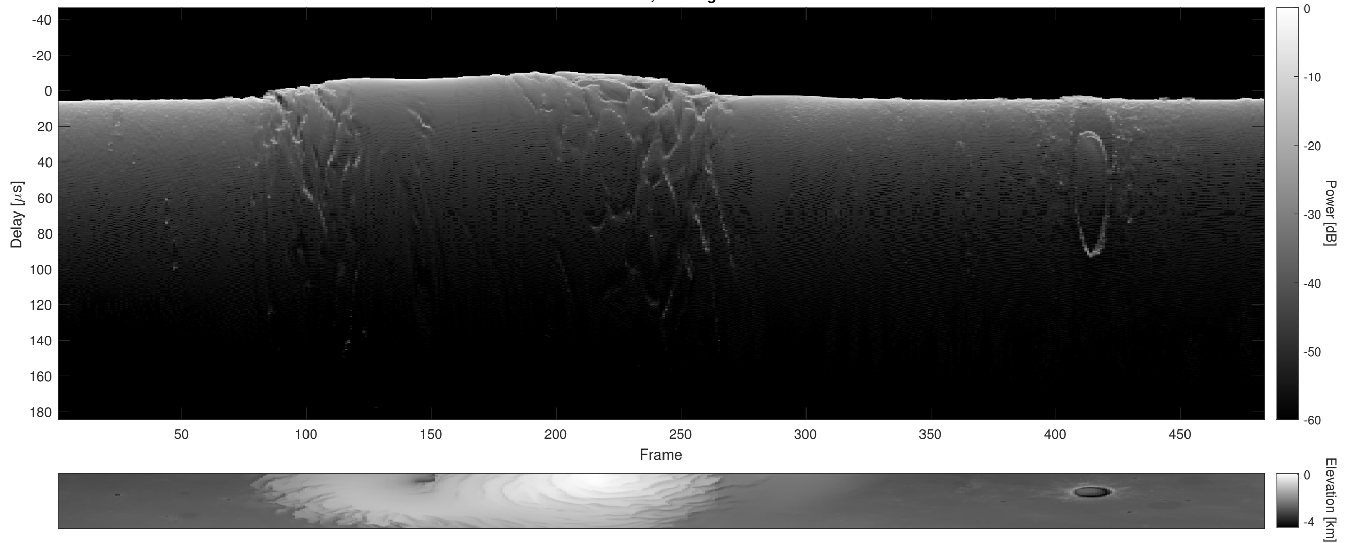
Orbit 5431, Cluttergram
