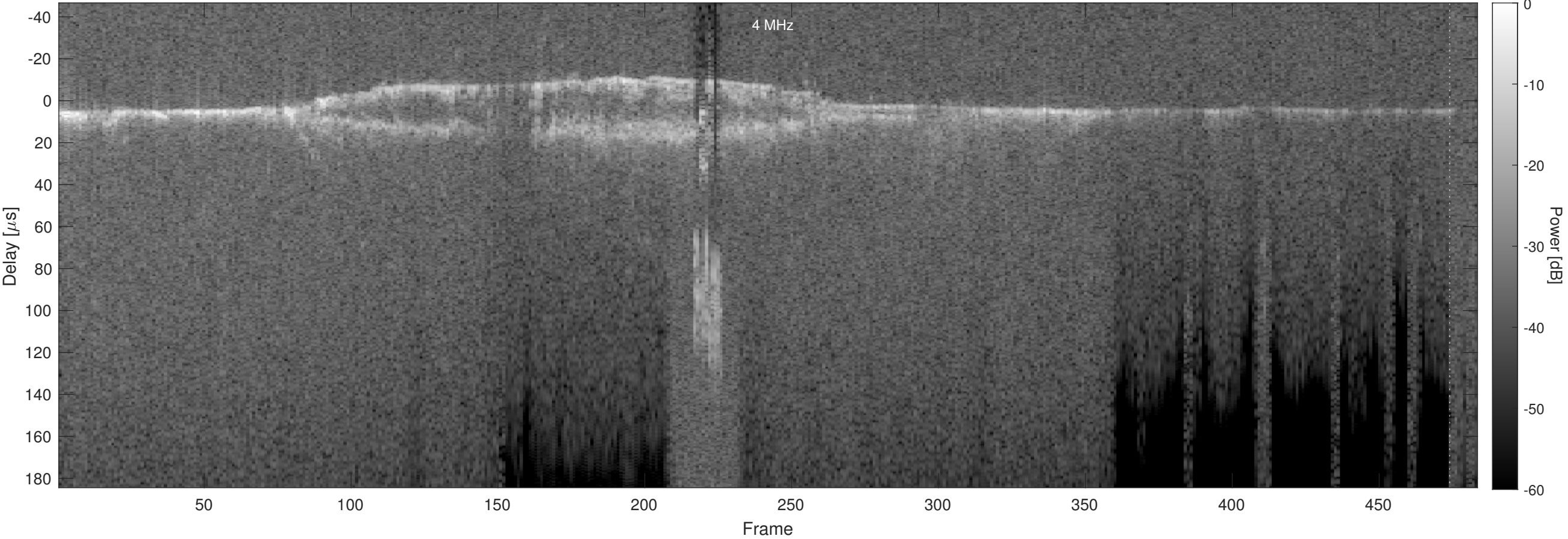
Orbit 5431, Optimized, No Window, Channel 2
