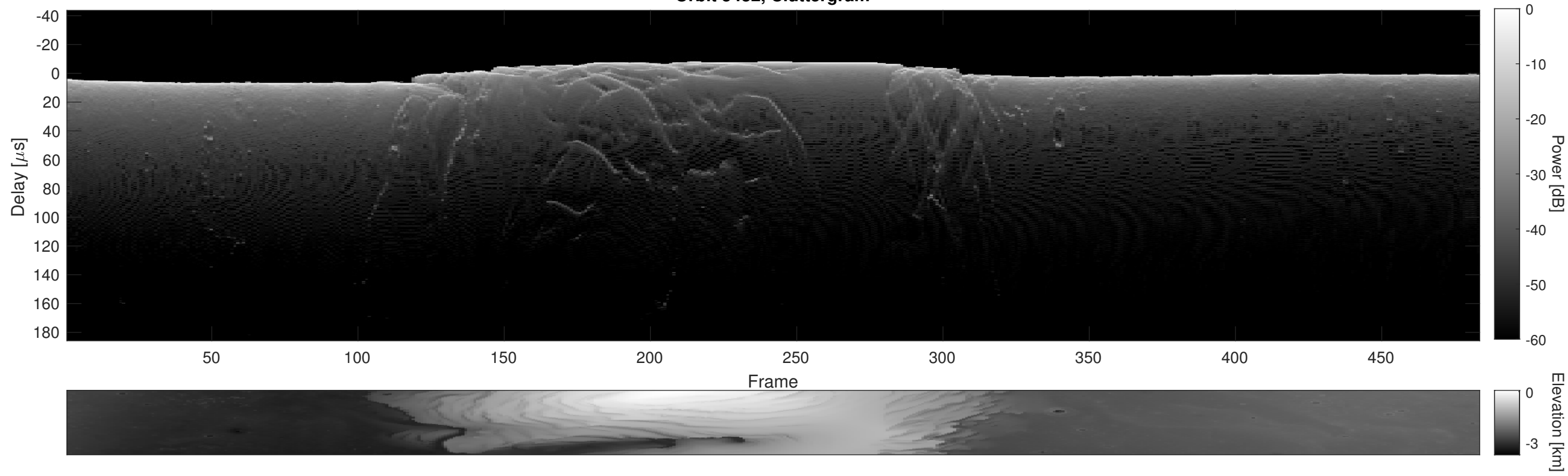
Orbit 5432, Cluttergram
