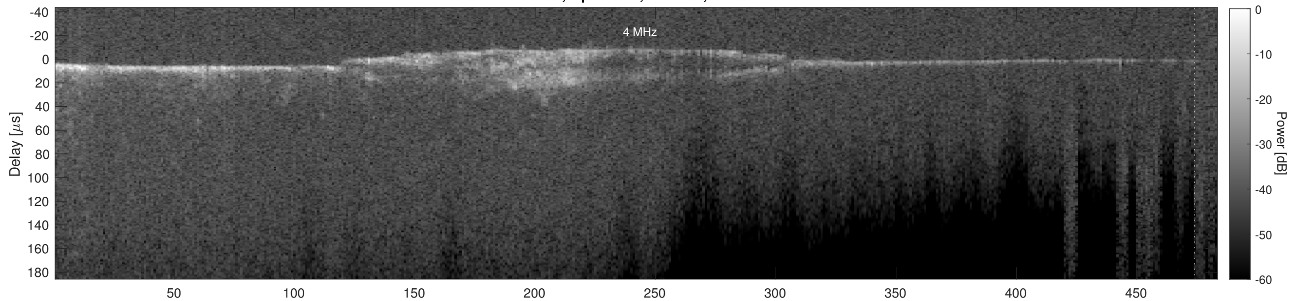
Orbit 5432, Cluttergram
