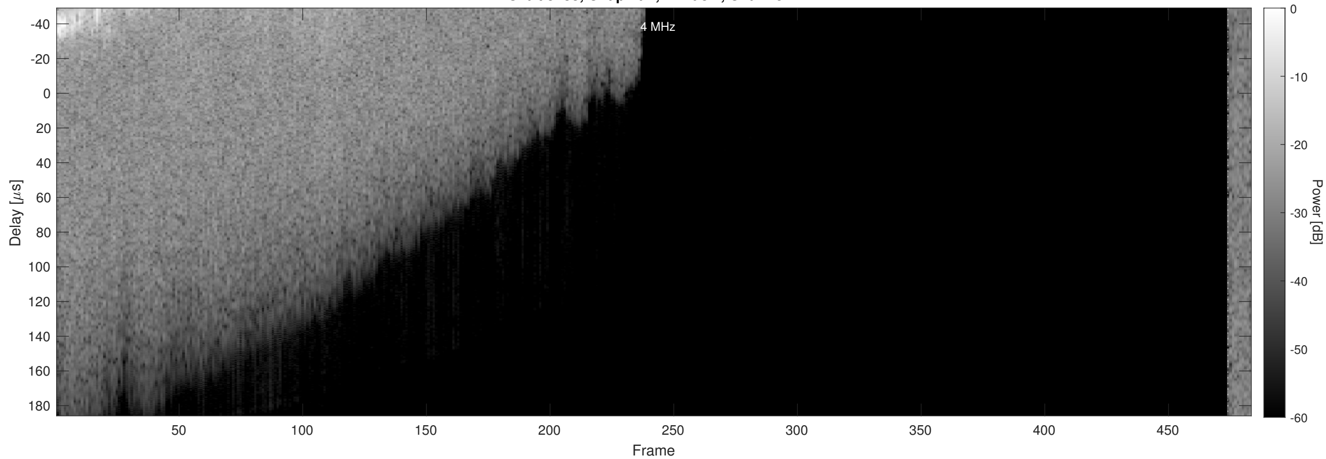
Orbit 5433, Chapman, Window, Channel 2
