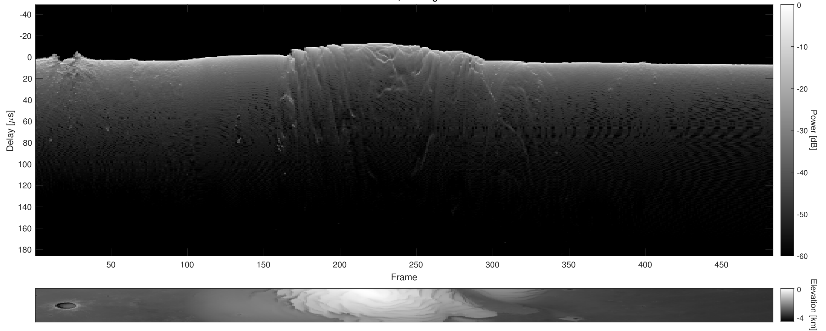
Orbit 5433, Cluttergram
