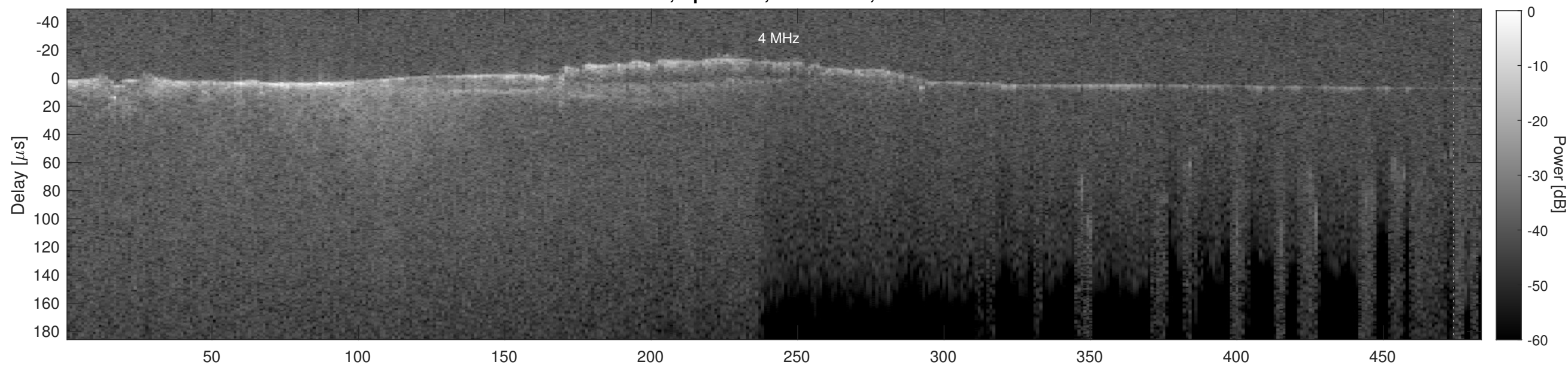
Orbit 5433, Cluttergram
