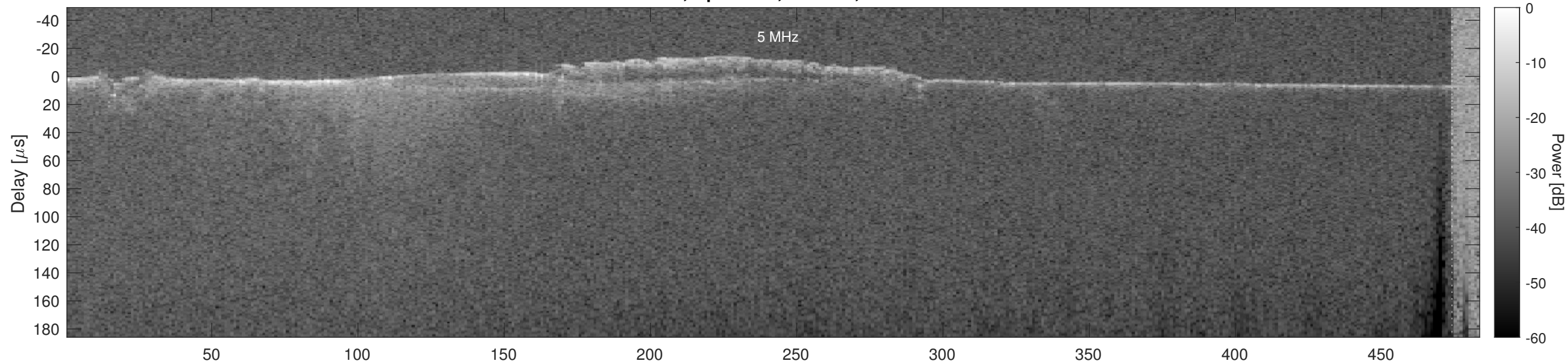
Orbit 5433, Optimized, Window, Channel 2
