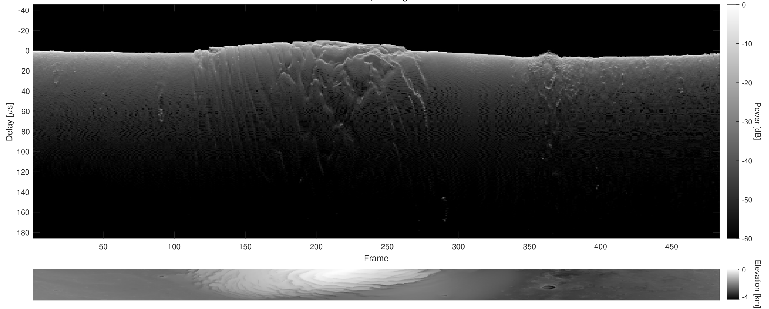
Orbit 5434, Cluttergram
