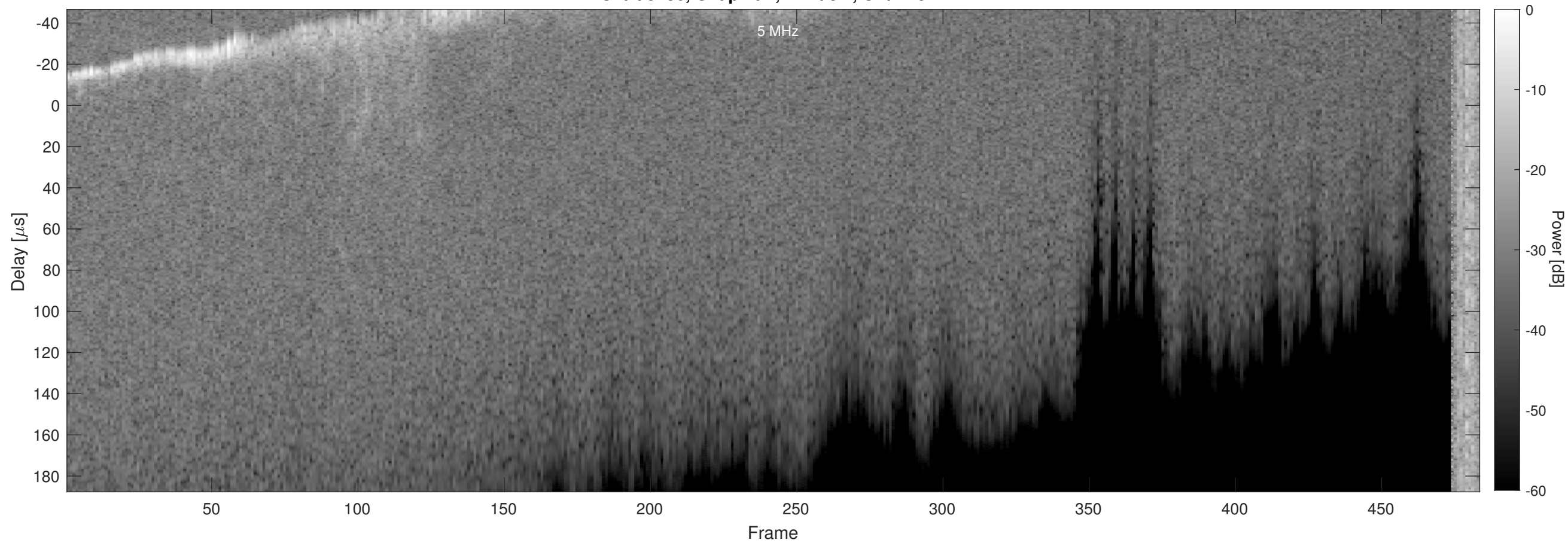
Orbit 5436, Chapman, Window, Channel 2
