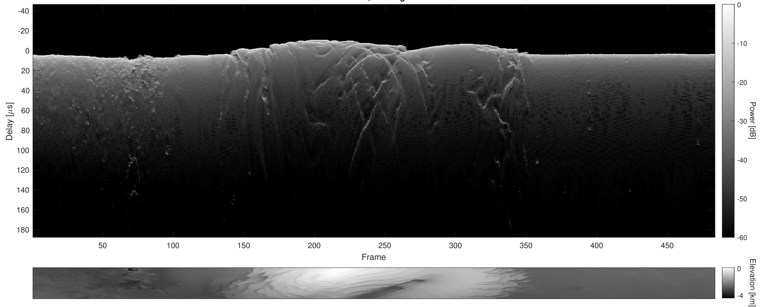
Orbit 5436, Cluttergram
