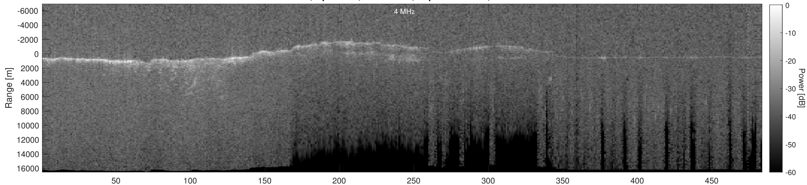
Orbit 5436, Depth-Corrected Cluttergram
