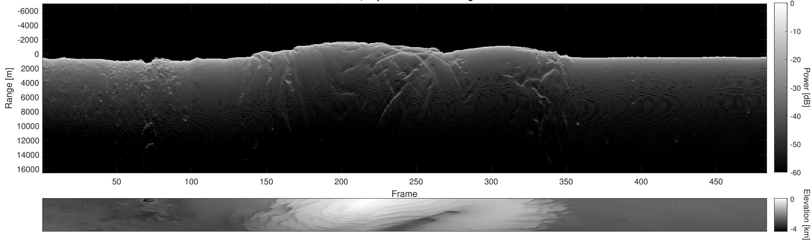
Orbit 5436, Depth-Corrected Cluttergram
