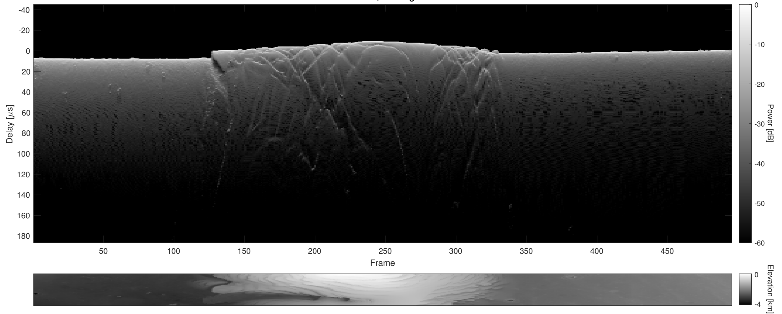
Orbit 5439, Cluttergram
