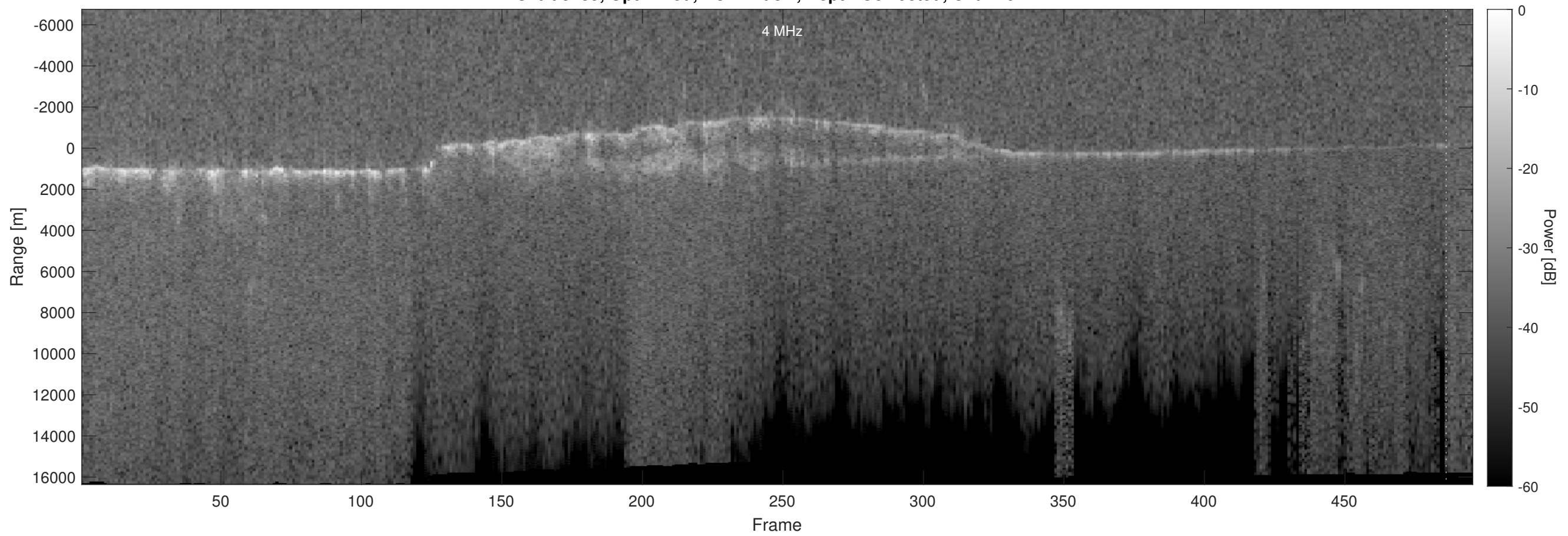
Orbit 5439, Optimized, No Window, Depth-Corrected, Channel 2
