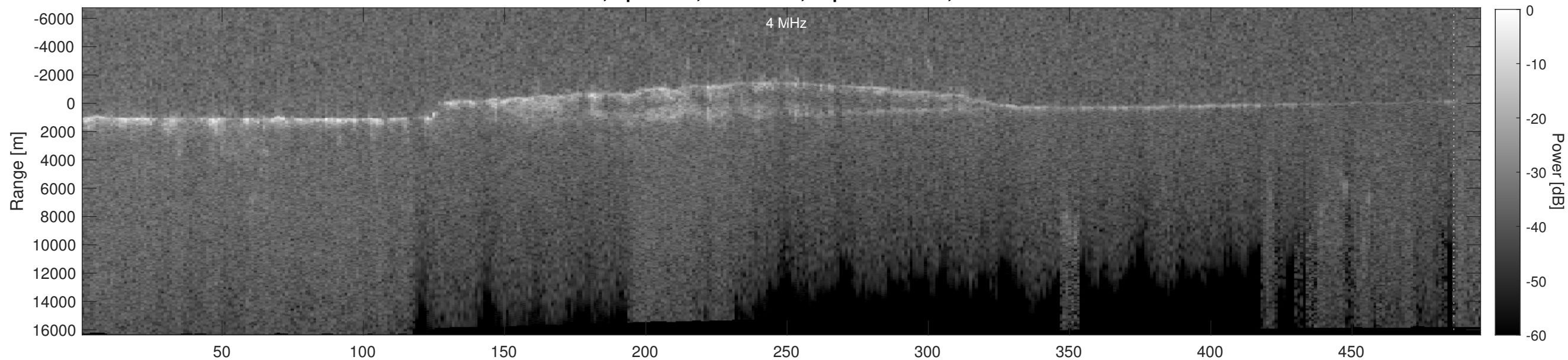
Orbit 5439, Depth-Corrected Cluttergram
