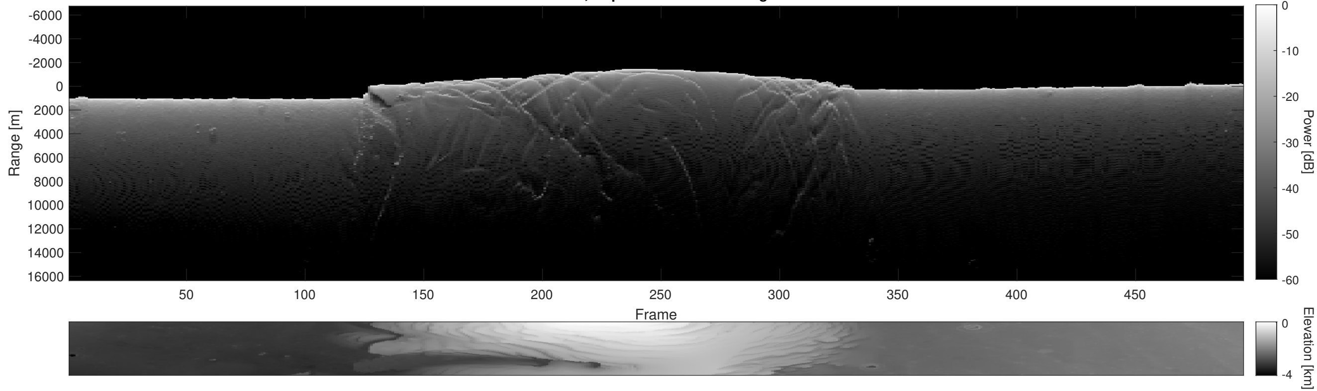
Orbit 5439, Depth-Corrected Cluttergram
