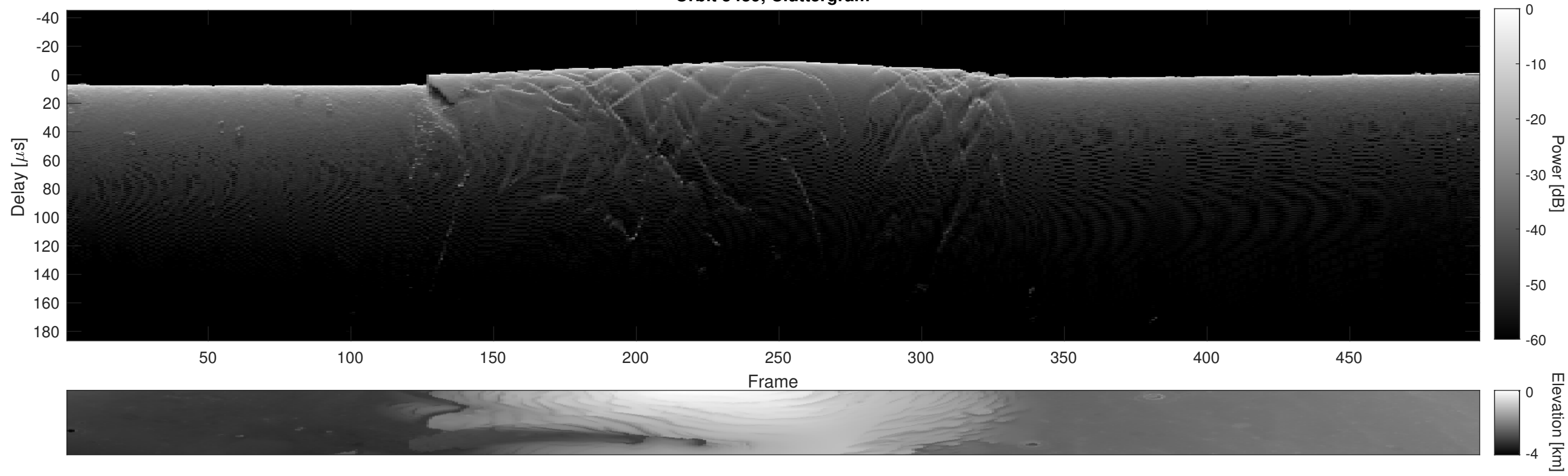
Orbit 5439, Cluttergram
