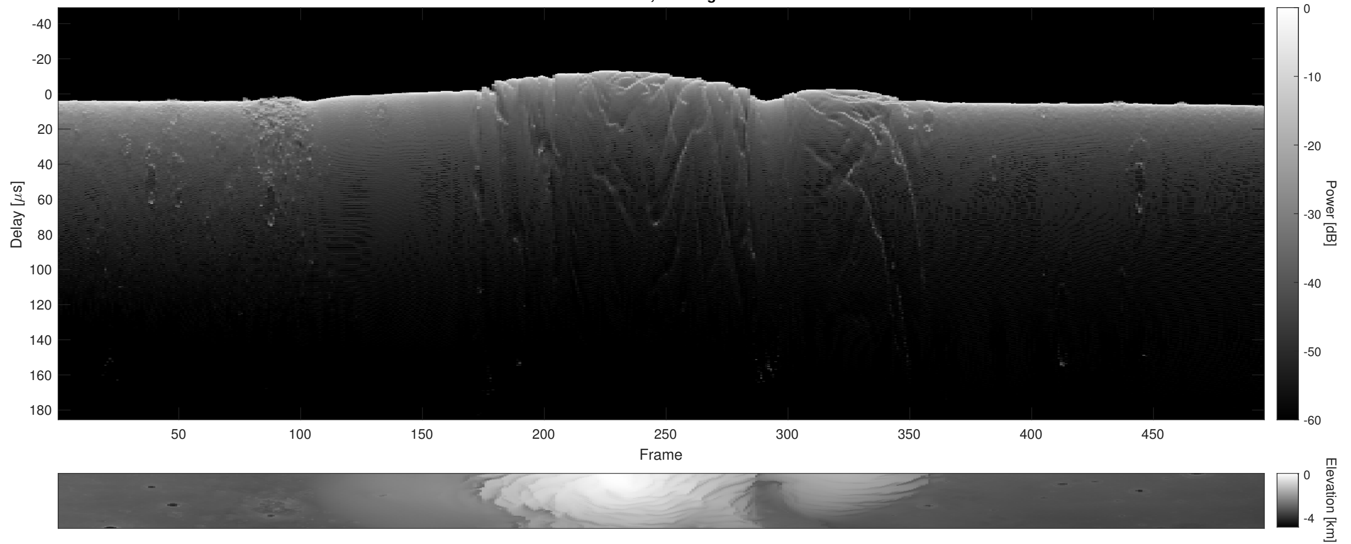
Orbit 5440, Cluttergram
