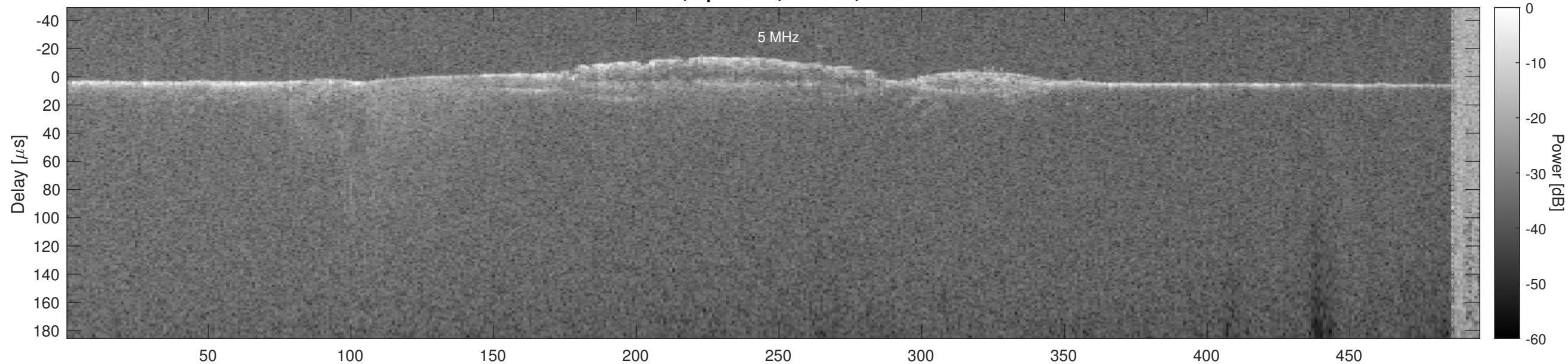
Orbit 5440, Optimized, Window, Channel 2
