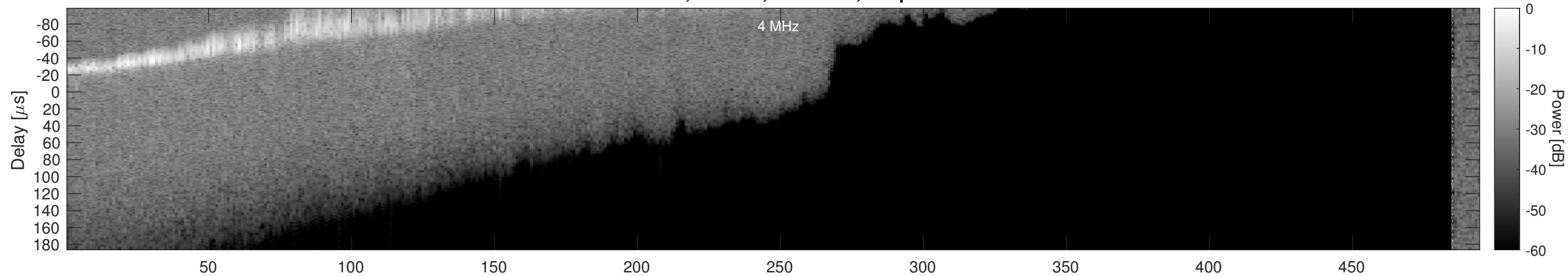
Orbit 5443, Window, Channel 2, Optimized
