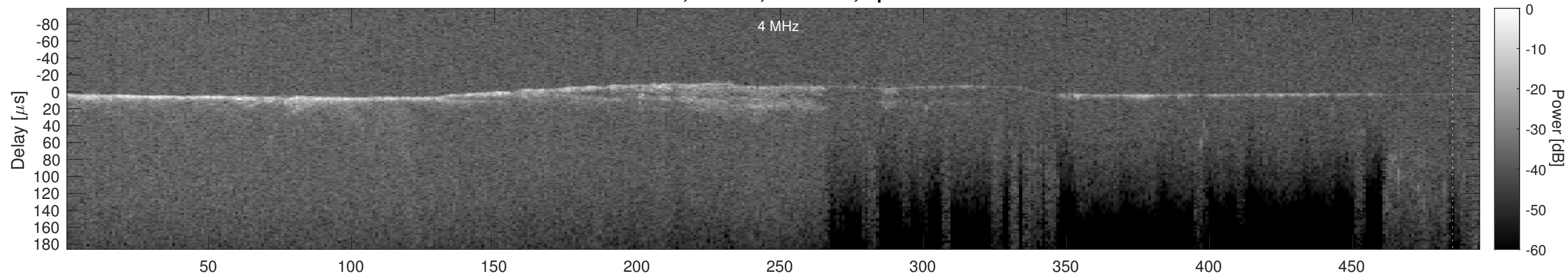
Orbit 5443, Cluttergram
