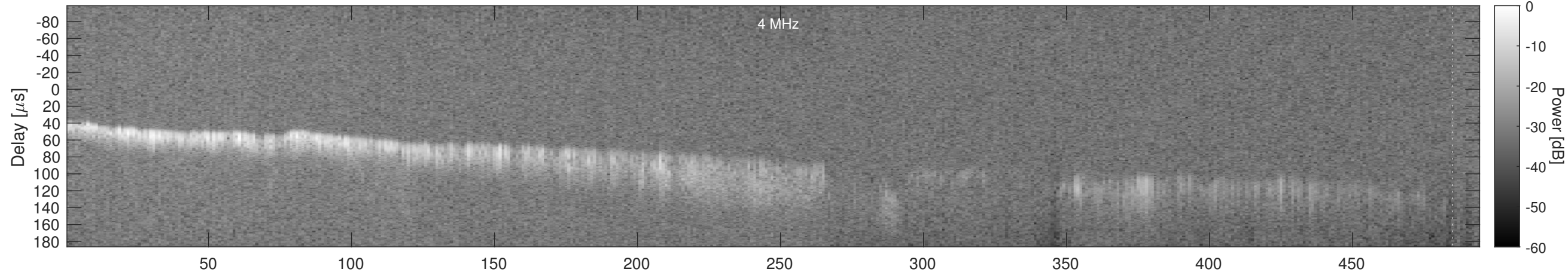
Orbit 5443, Window, Channel 2, Chapman
