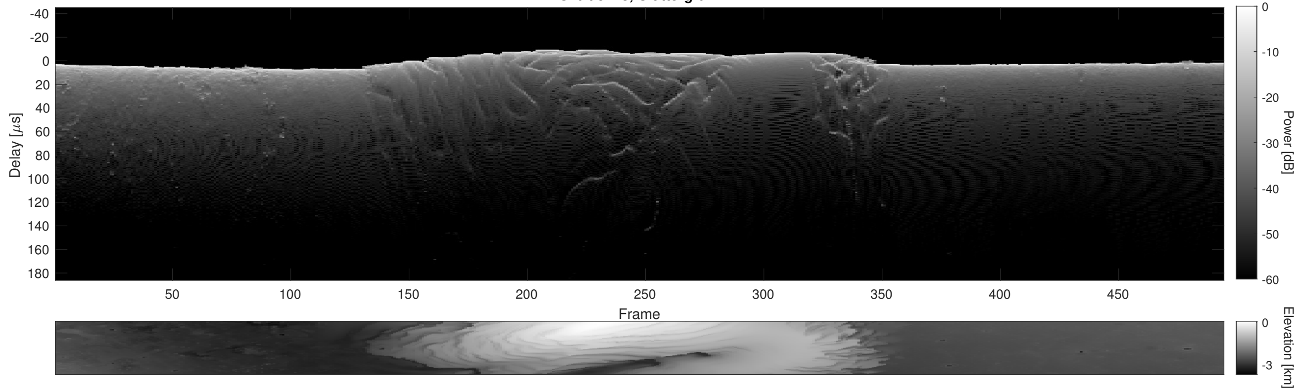
Orbit 5443, Cluttergram
