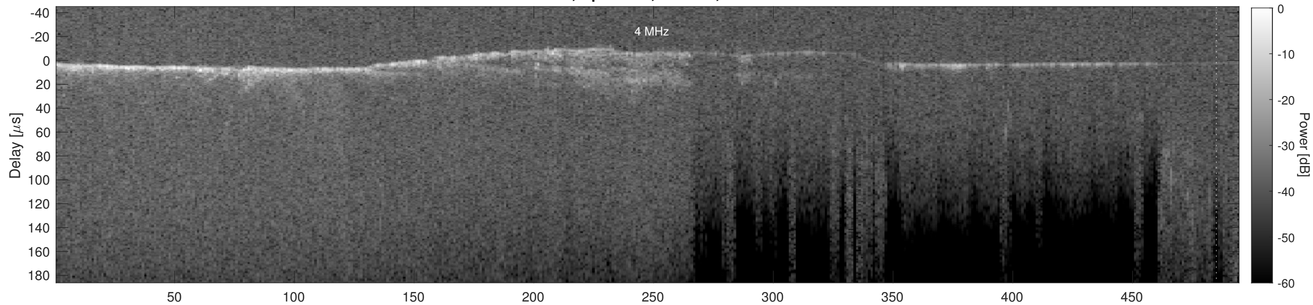
Orbit 5443, Cluttergram
