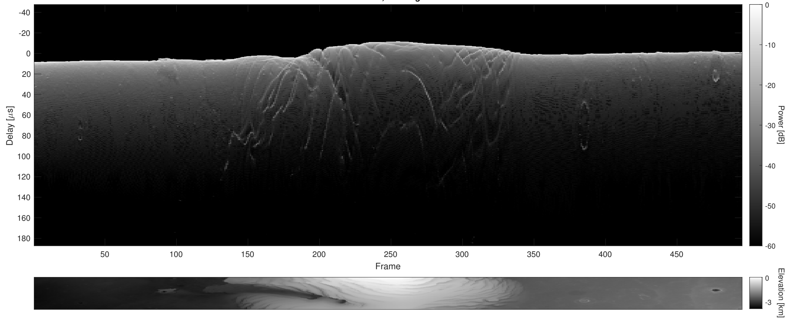
Orbit 5446, Cluttergram
