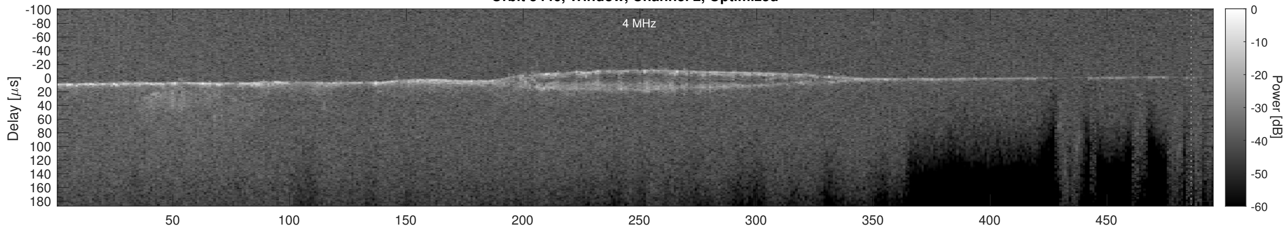
Orbit 5446, Cluttergram
