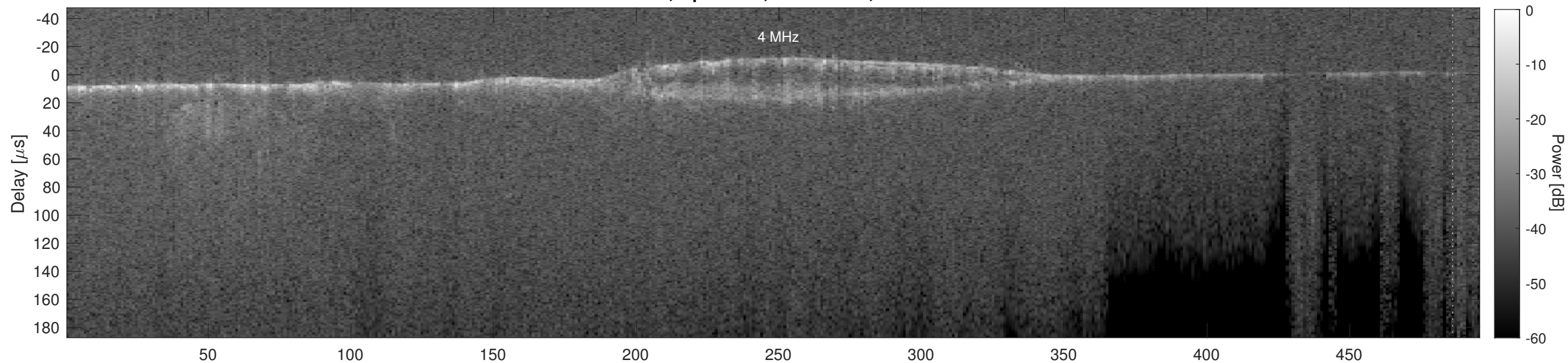
Orbit 5446, Cluttergram
