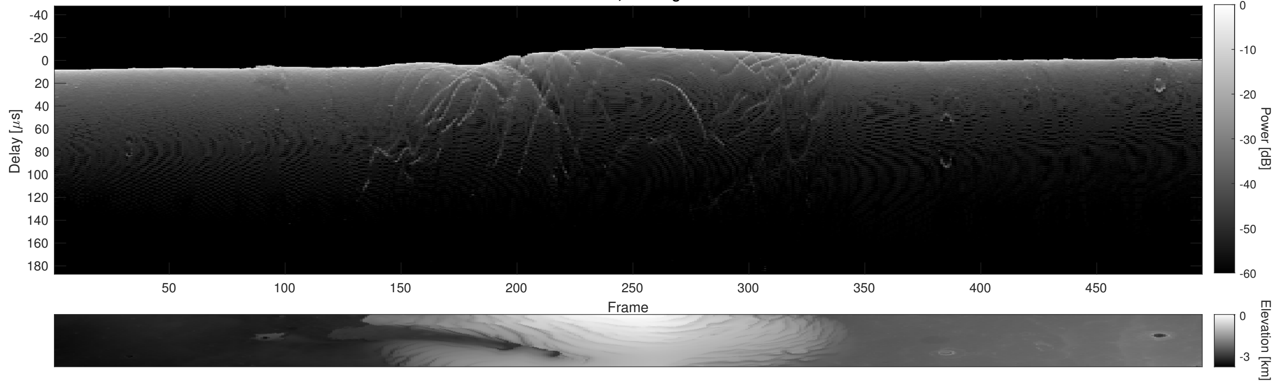
Orbit 5446, Cluttergram
