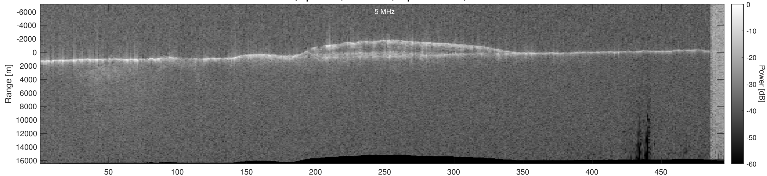
Orbit 5446, Optimized, No Window, Depth-Corrected, Channel 2
