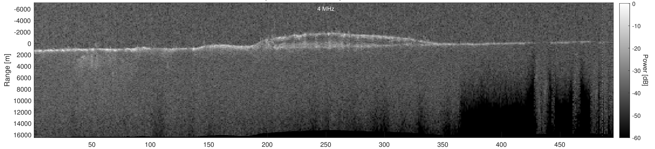
Orbit 5446, Depth-Corrected Cluttergram
