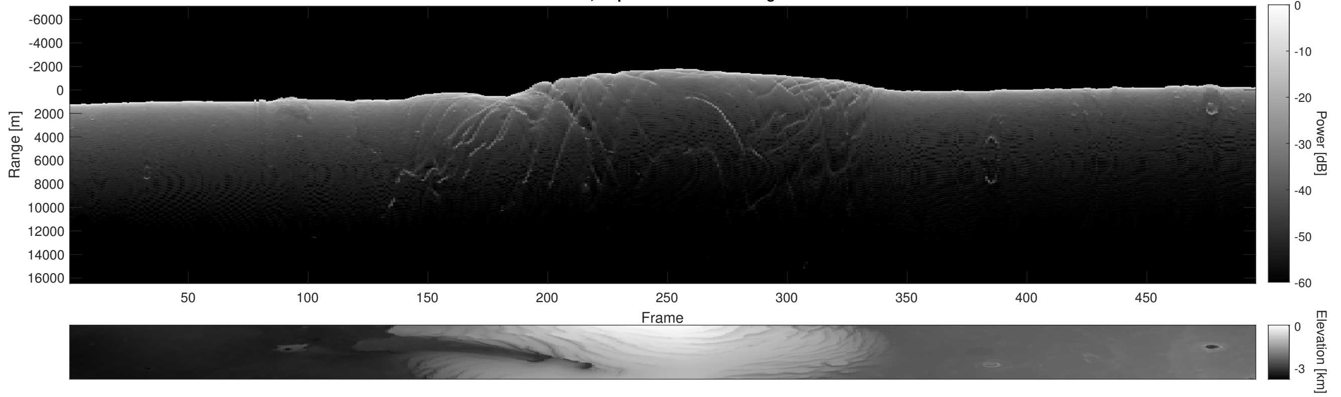
Orbit 5446, Depth-Corrected Cluttergram
