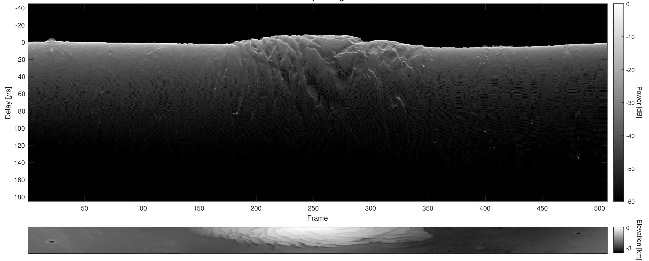
Orbit 5448, Cluttergram
