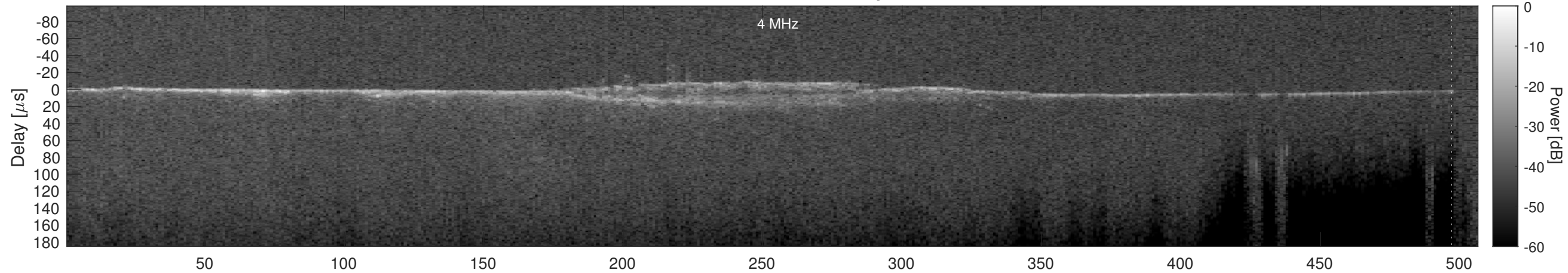
Orbit 5448, Cluttergram
