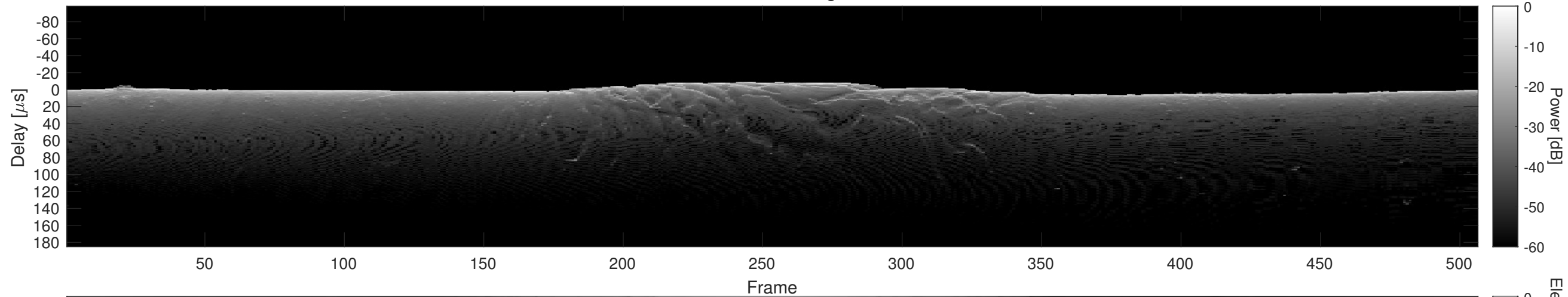
Orbit 5448, Cluttergram
