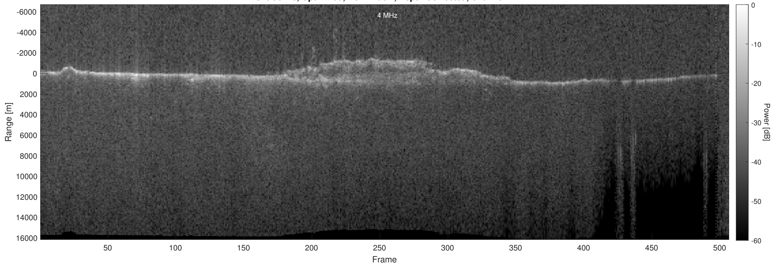
Orbit 5448, Optimized, No Window, Depth-Corrected, Channel 2
