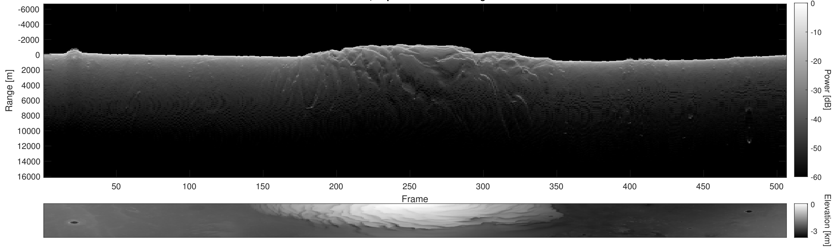
Orbit 5448, Depth-Corrected Cluttergram
