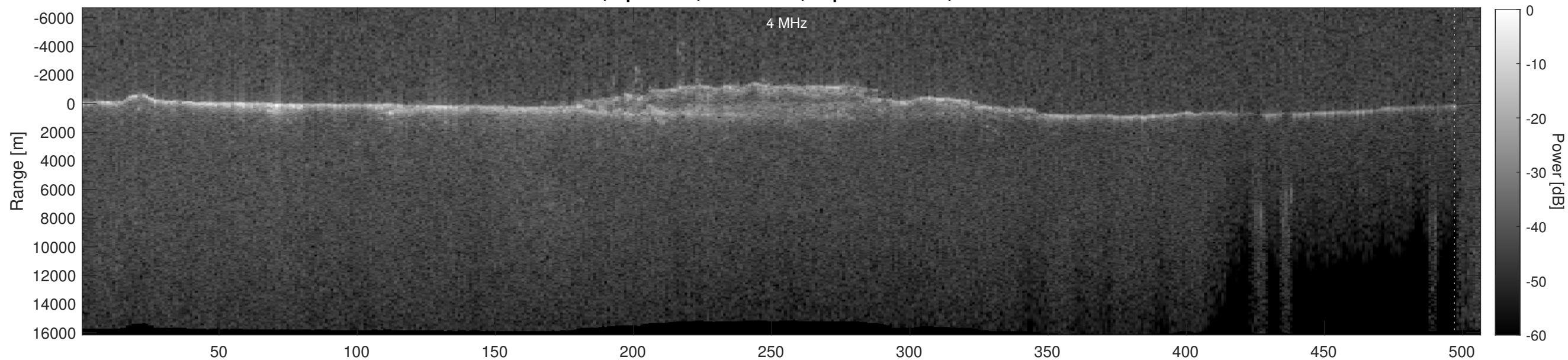
Orbit 5448, Depth-Corrected Cluttergram
