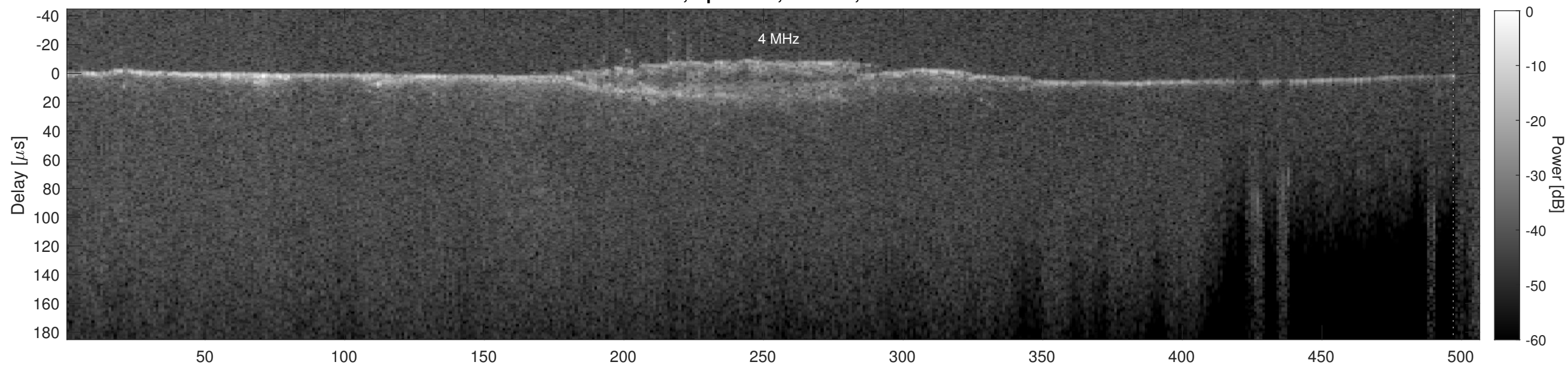
Orbit 5448, Cluttergram
