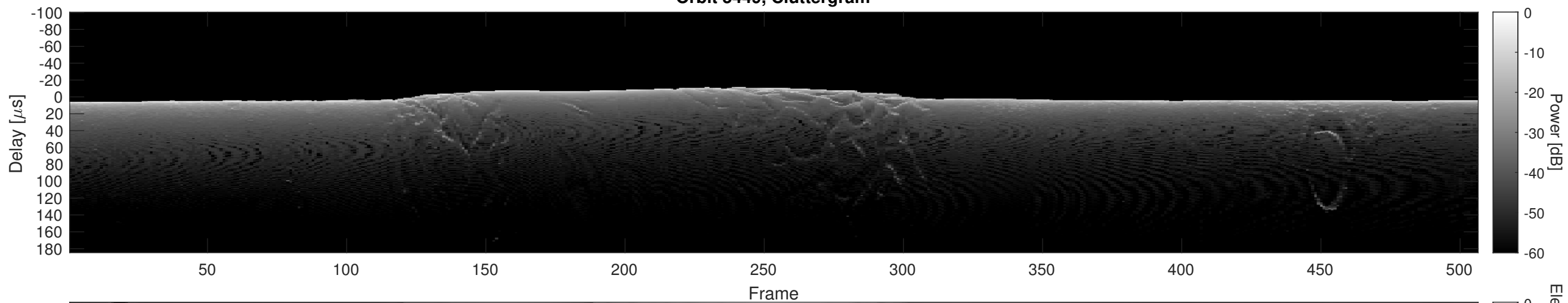
Orbit 5449, Cluttergram
